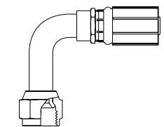
JIC 37° FJX90L
